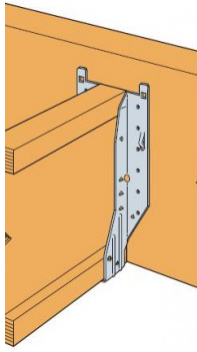
Face fix to solid joist.
